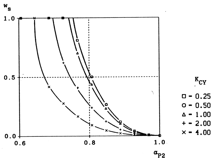
Fig. 4. Variation of the sol fraction, w_s , with \alpha_{P2} = (3)\alpha_c for K_{CY} = 0.25; 0.50; 1.00; 2.00 and 4.00 , Y = E, F .
