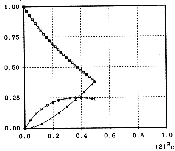
Fig. 2. Variation of q_0 , q_1 and q_2 with (2)\alpha_c for K_{cy} = 1 (left) and K_{cy} = 4 (right), Y = D, T .
