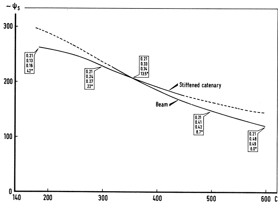
Figure 4. Maximum bending stress / cable length for pipe of fig. 3, with D_{sh} = 150 and H = 140 . Boxed numbers: \epsilon , \epsilon\kappa/\mu , \epsilon/\mu , maximum angle.
