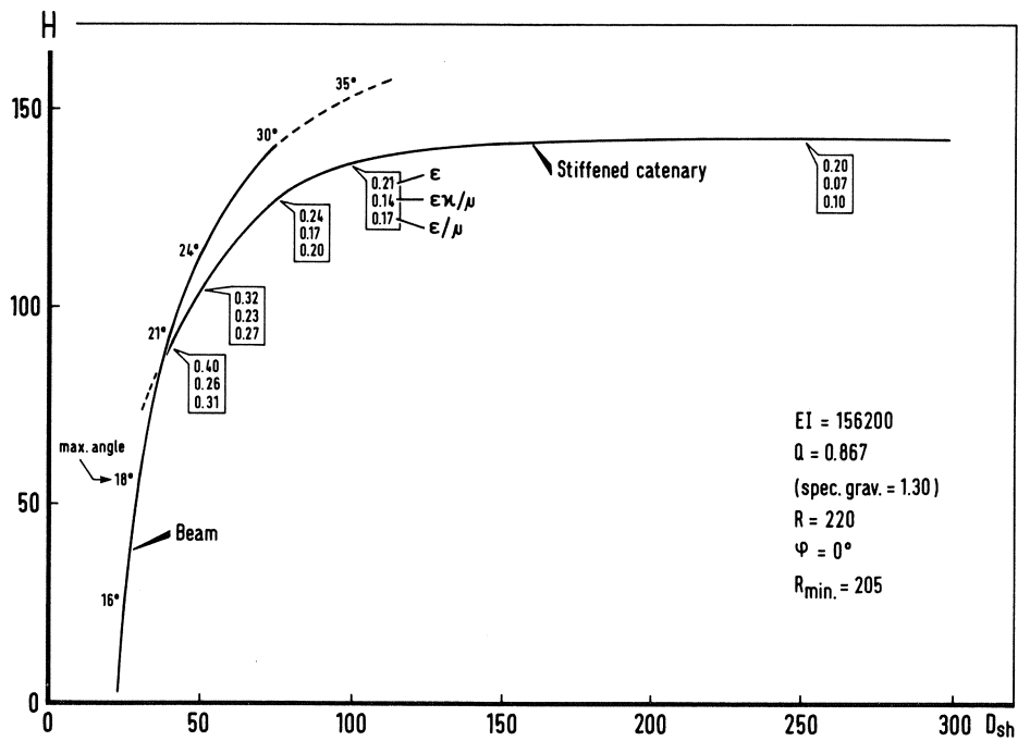
Figure 3. Tension / waterdepth diagram for constant minimum radius of curvature ( R_{min} )
