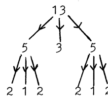
DEN(H(\frac{5}{13}))
