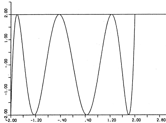
Figure 6: \Delta_q for b=0 (here q=7 ).
