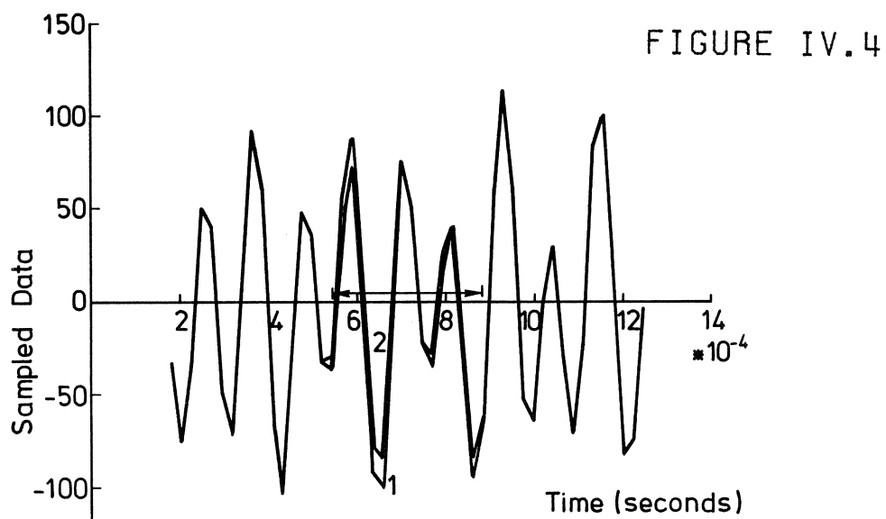
Fig. IV.4 Restoration result and original signal for an autoregressive process with a peaky spectrum, m=16 , p=10 , N=64 , after 1 iteration. Restoration error e=0.38E-01 .
