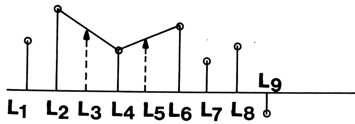
Fig. 10. First-order linear interpolation
