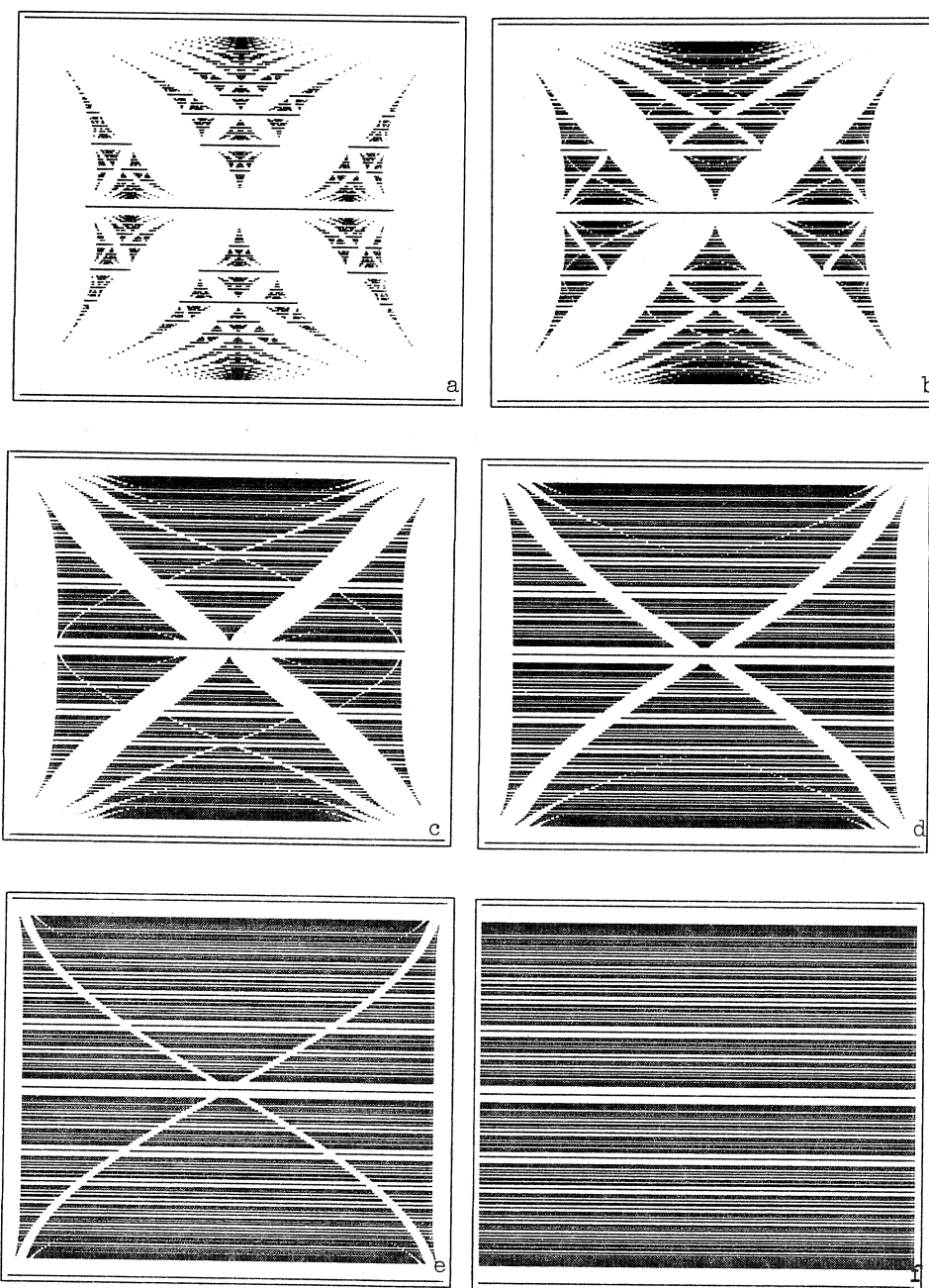
Figure 1: Hofstadter pictures. a A=1.0 b A=0.6 c A=0.3 d A=0.15 e A=0.06 f A=0.0 . Abscissa: \text{spect}(A, \alpha) . Ordinate: 0 \leq \alpha \leq 1 .
