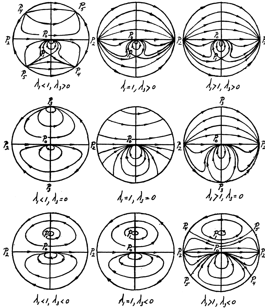
figure 6 : \lambda_2 = 0
