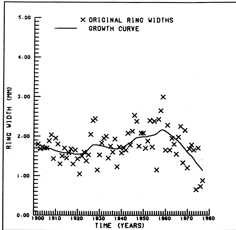
Figure 1. Ring width series in mm of a European silver fir ( Abies alba Mill.), cut in Wörth (GFR) in 1978. The length of the series N = 78 . The solid line represents the trend g_t or growth curve as estimated by the model and filtering methods explained in the text.
