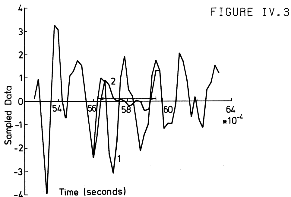
Fig. IV.3 Restoration result and original signal for an autoregressive process with a smooth spectrum, m=16 , p=10 , N=512 , after 1 iteration. Restoration error e=0.10E+01 .
