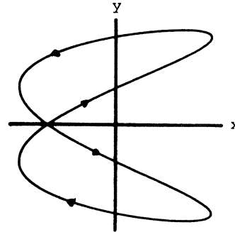
Fig. 4.4. \theta = \frac{\pi}{4}
